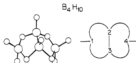
Figure 3. Geometrical and localized valence structure of B 4 H 10 . One terminal hydrogen is omitted from each boron (or, later, carbon) atom. The extra terminal H is indicated by a straight line, and the bridge hydrogen by a curved line.
